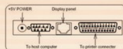
Connector Panel
